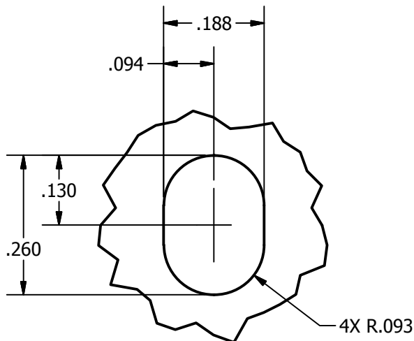
DETAIL A SLOT 4 PLACES
